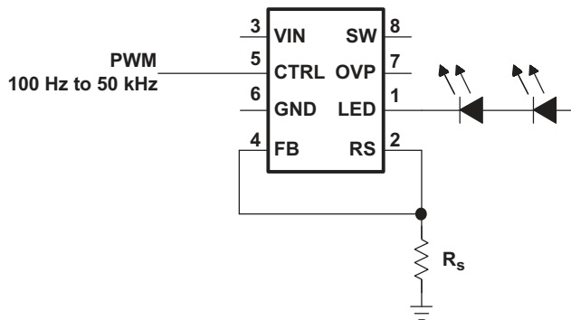
Figure 10. Setting the LED Current
