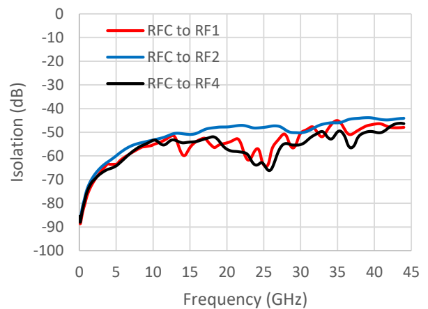
Isolation between RF1 to RF4, RFC to RF2 On 11
