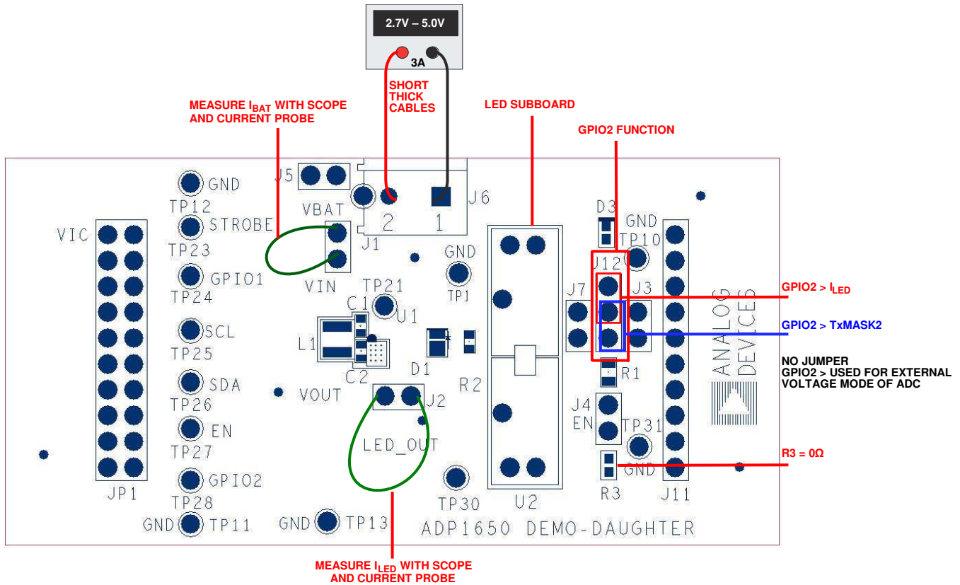
Figure 10. Demonstration Daughterboard
