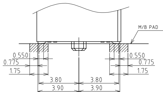
SOLDERING DIM DETAIL 3:1
