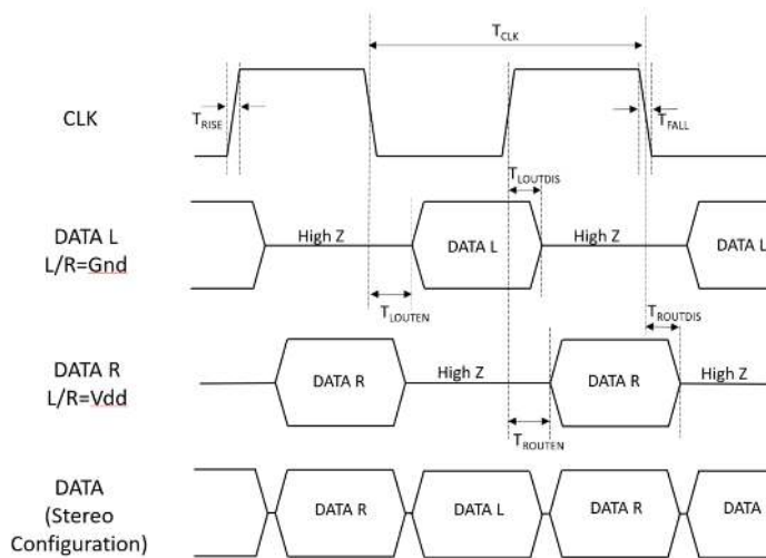
Timing Diagram for CLK, DATA L, DATA R in Stereo Configuration
