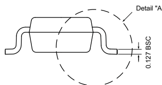
End View
