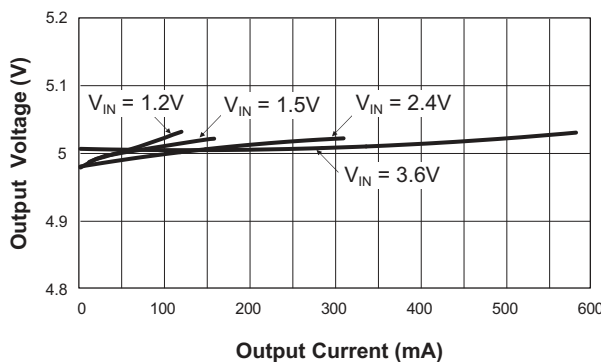
Output Voltage vs. Output Current ( V_{OUT} = 5V ; T_A = 25^\circ C )
