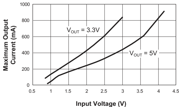
Maximum Output Current vs. Input Voltage ( L = 4.7\mu H ; T_A = 25^\circ C )
