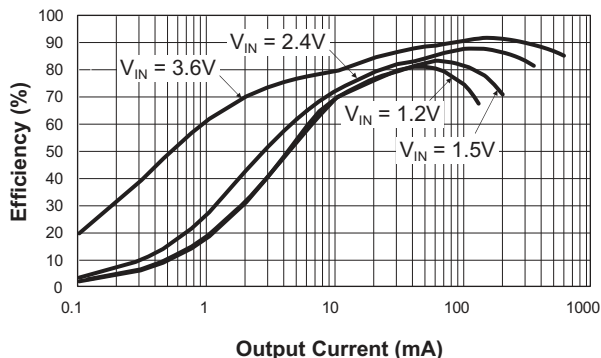
Efficiency vs. Output Current ( V_{OUT} = 5V ; T_A = 25^\circ C )
