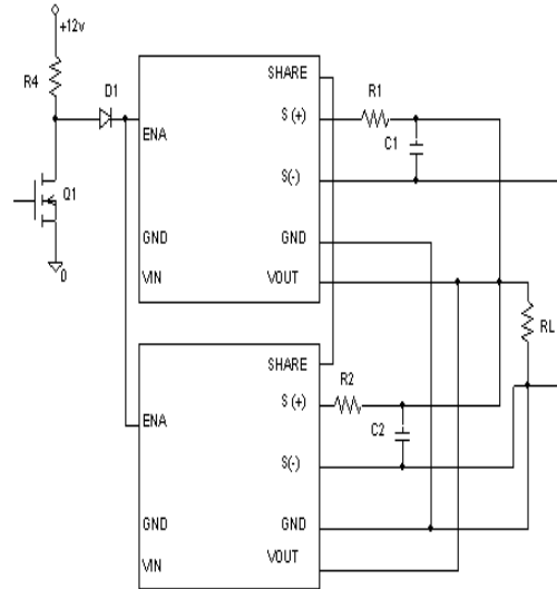
Figure 28. Circuit Configuration for modules in parallel.
