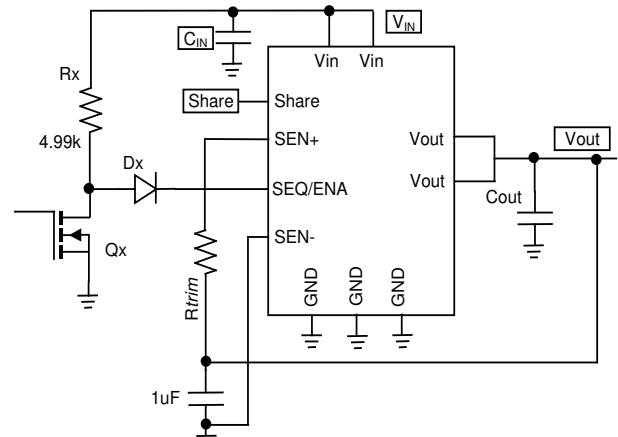
Figure 24. Application Schematic
