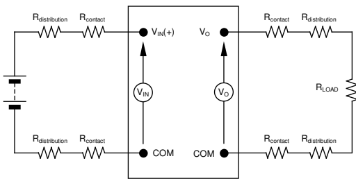
Figure 22. Output Ripple and Noise Test Setup.
