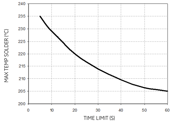
Figure 33. Time Limit Curve Above 205°C Reflow.
