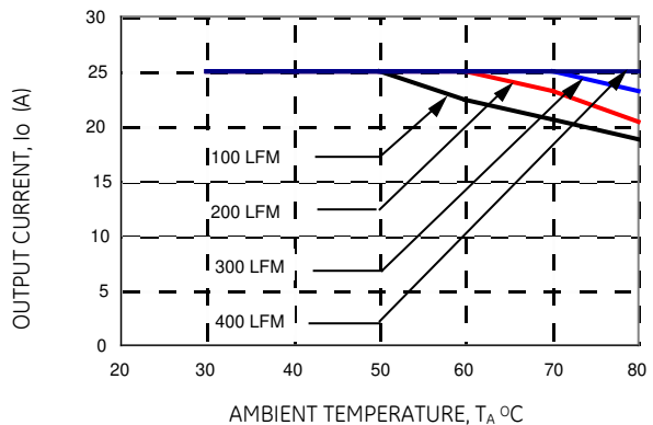
Figure 20. Derating Output Current versus Local Ambient Temperature and Airflow (Vin = 12Vdc, Vo=5.0 Vdc) with baseplate.
