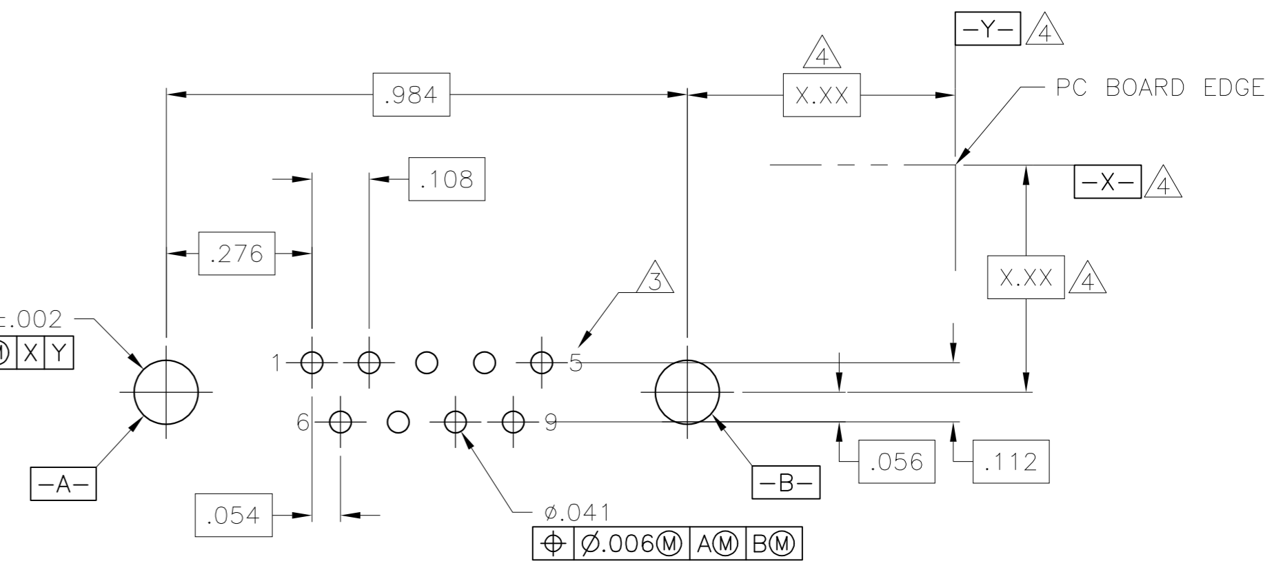
RECOMMENDED PC BOARD LAYOUT .062 PC BOARD (VIEWED FROM CONNECTOR SIDE)
