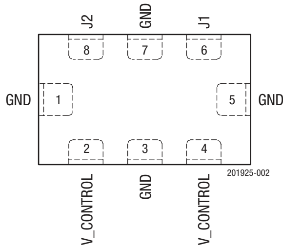
Figure 2. SKY12233-11 Pinout (Top View)
