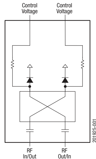
Figure 1. SKY12233-11 Block Diagram
