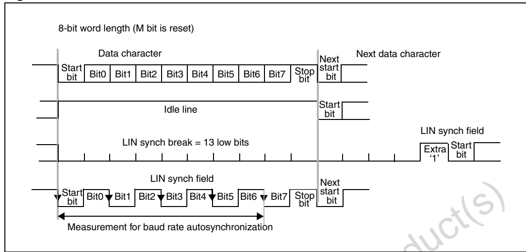
Figure 59. LIN characters
