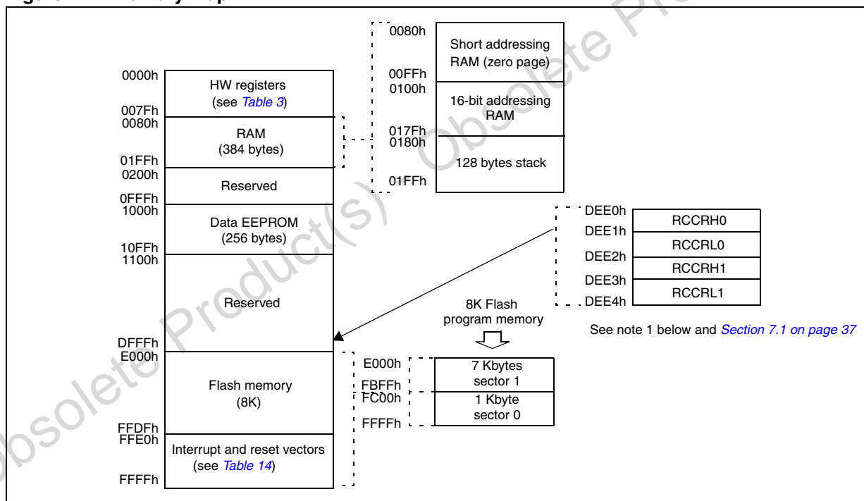
Figure 4. Memory map
