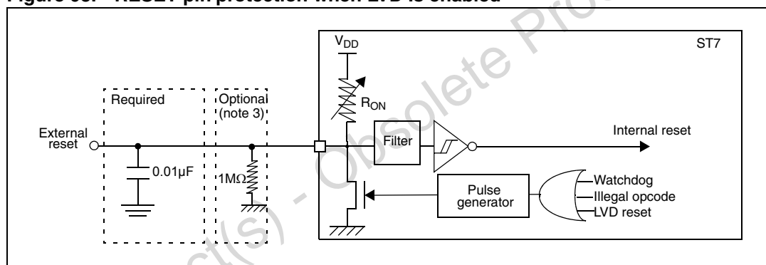
Figure 98. RESET pin protection when LVD is enabled
