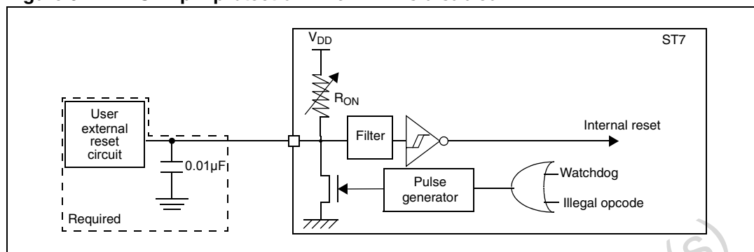
Figure 97. RESET pin protection when LVD is disabled
