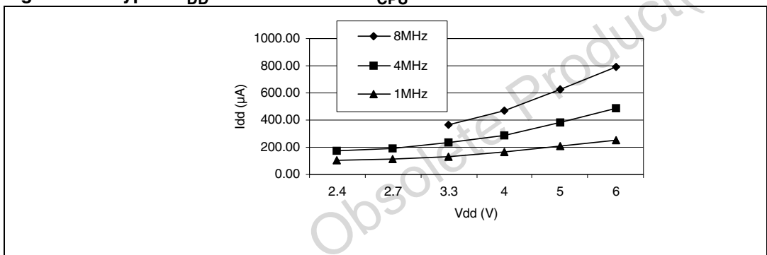
Figure 80. Typical I_{DD} in wait mode vs. f_{CPU}
