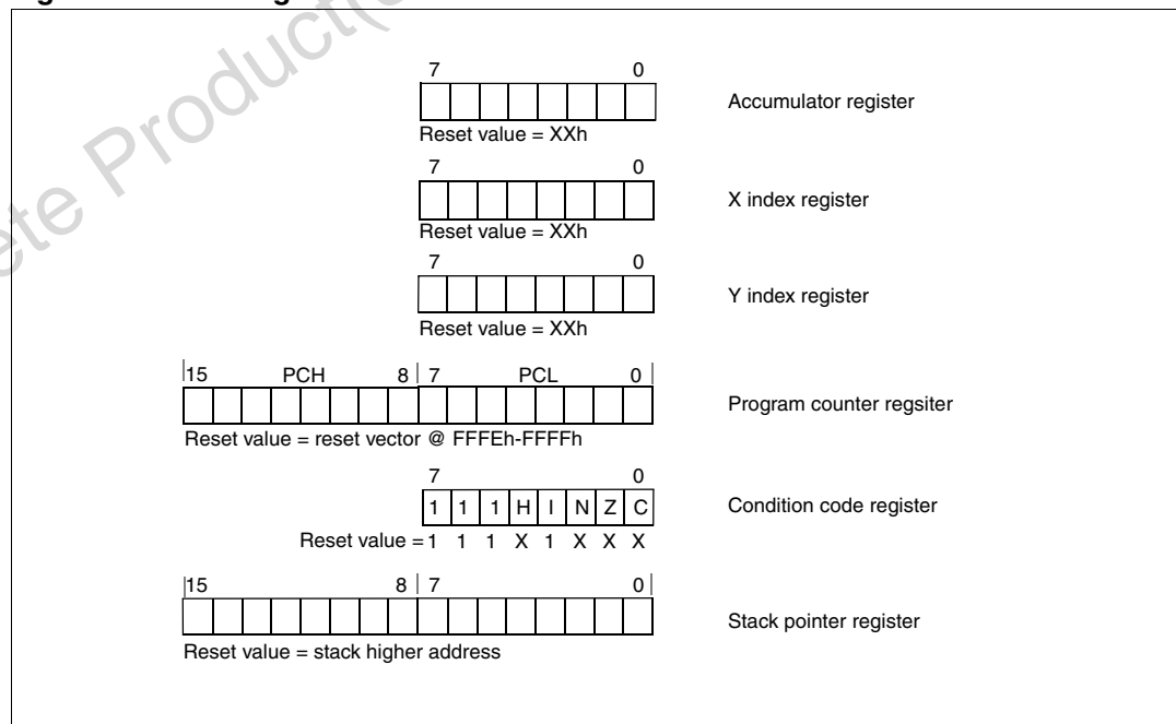
Figure 10. CPU registers
