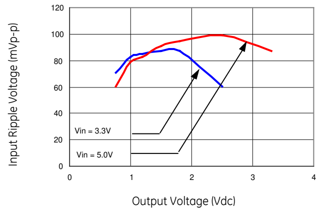
Figure 26. Input ripple voltage for various output with 1 \times 150 \mu F polymer and 1 \times 47 \mu F ceramic capacitors at the input (80% of I_{O,max} ).
