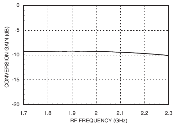
Unconverter Performance Conversion Gain @ LO = +17 dBm
