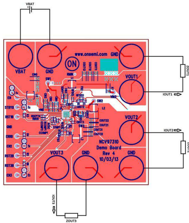
Figure 5. NCV97310 Board Connections
