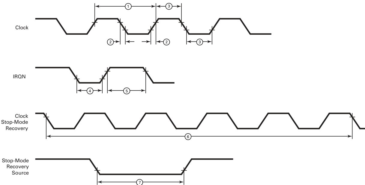
FIGURE 5. ADDITIONAL TIMING
