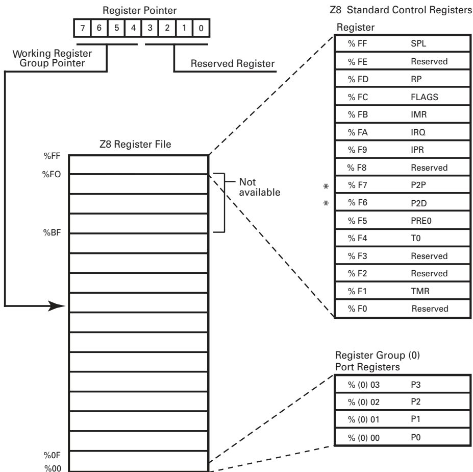
FIGURE 11. REGISTER FILE ARCHITECTURE
