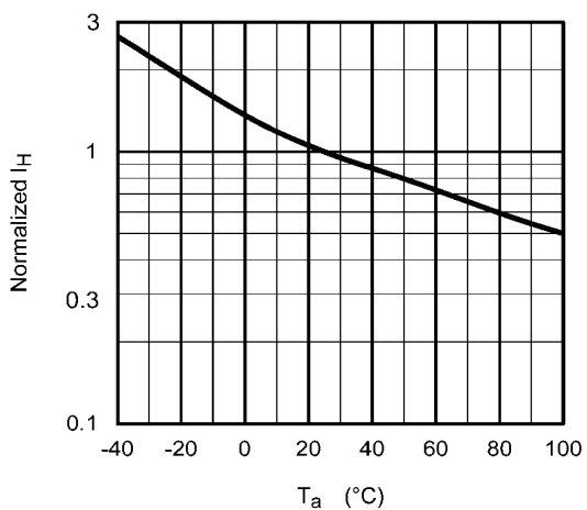
Fig. 12.9 Normalized I_H - T_a
