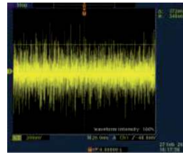
Measurement of PE ground noise in a machine with VFDs on
