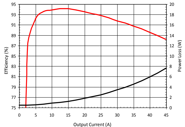
Figure 2: Typical IR3558 Efficiency & Power Loss (See Note 2 on Page 7)
