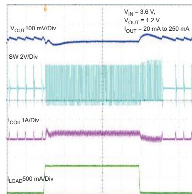
Time Base - 10 µs/Div
