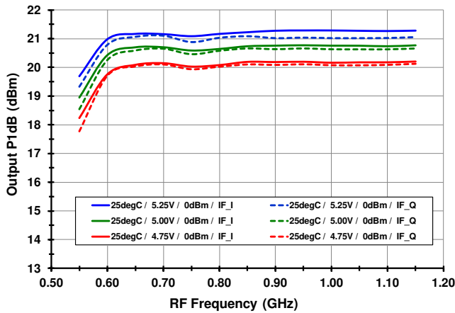
P1dB O vs. V CC [ Low Side Injection]
