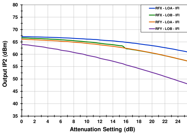
IP2 O [0.8 GHz RF, HiSide Inj.]
