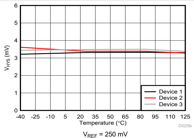
Figure 6-16. Cmp0 Trip Threshold Hysteresis vs Temperature
