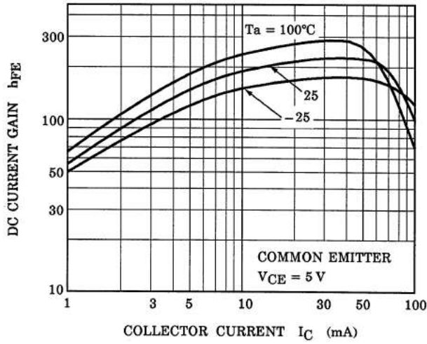
Fig. 10.7 RN1907 h_{FE}-I_C
