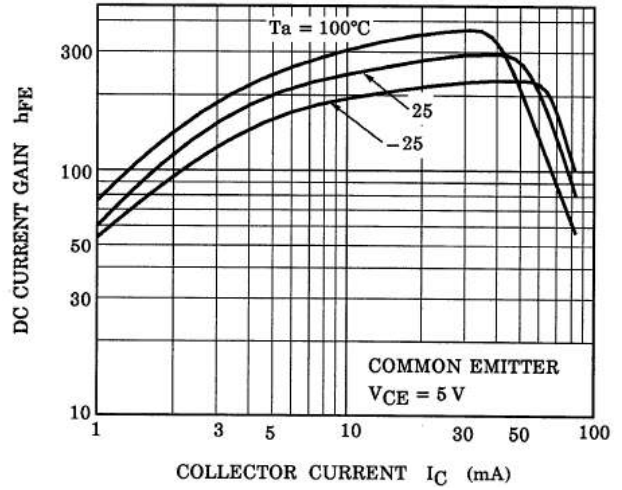
Fig. 10.8 RN1908 h_{FE}-I_C
