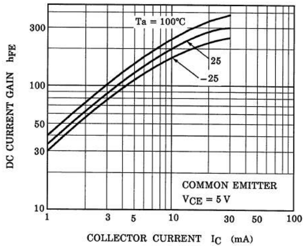
Fig. 10.9 RN1909 h_{FE}-I_C
