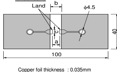
Fig.1 (in mm)
