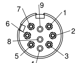
FACE VIEW SF3282-6ASG-5XX POS. 4, 8 & 9 MOLDED HALF CLOSED
