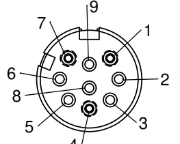
FACE VIEW SF3282-3ASG-5XX POS. 2, 3, 5, 6, 8 & 9 MOLDED HALF CLOSED
