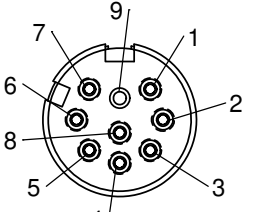
FACE VIEW SF3282-8ASG-5XX POS. 9 MOLDED HALF CLOSED
