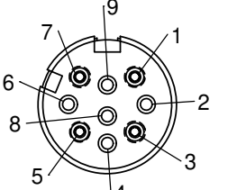
FACE VIEW SF3282-4ASG-5XX POS. 2, 4, 6, 8 & 9 MOLDED HALF CLOSED
