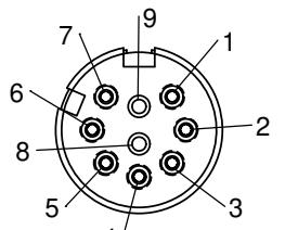
FACE VIEW SF3282-7ASG-5XX POS. 8 & 9 MOLDED HALF CLOSED
