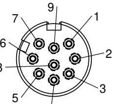
FACE VIEW SF3282-9ASG-5XX
