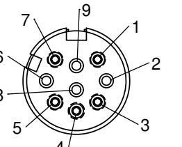
FACE VIEW SF3282-5ASG-5XX POS. 2, 6, 8 & 9 MOLDED HALF CLOSED
