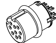
FACE VIEW SF3282-7ASG-5XX POS. 8 & 9 MOLDED HALF CLOSED
