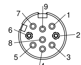
FACE VIEW SF3282-2ASG-5XX POS. 1, 3, 4, 5, 7, 8, & 9 MOLDED HALF CLOSED
