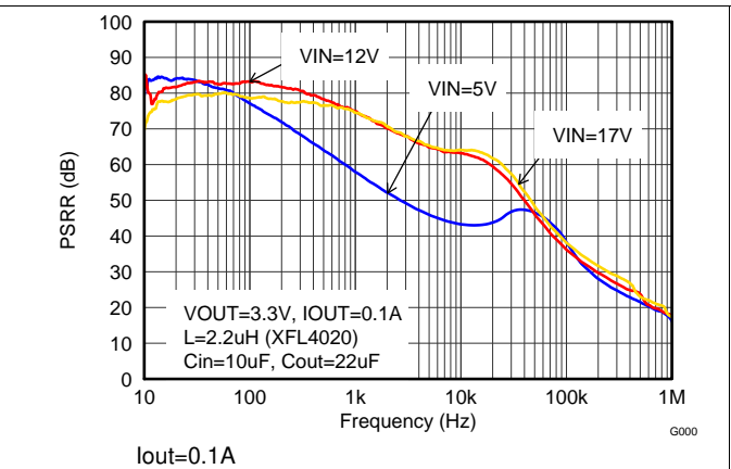
Figure 27. Power Supply Rejection Ratio, F_{SW} = 2.5\text{ MHz}
