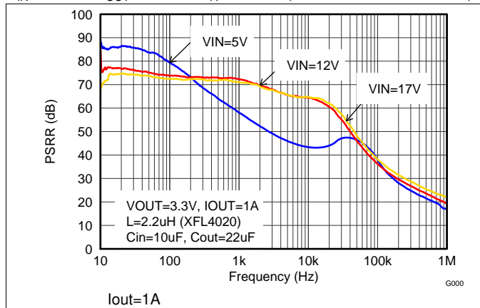
Figure 26. Power Supply Rejection Ratio, F_{SW} = 2.5\text{ MHz}
