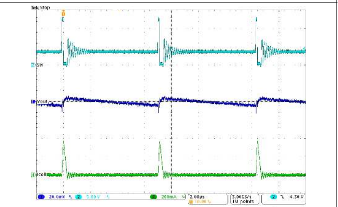
Figure 35. Typical Operation in Power Save Mode ( I_{OUT} = 10\text{ mA} )
