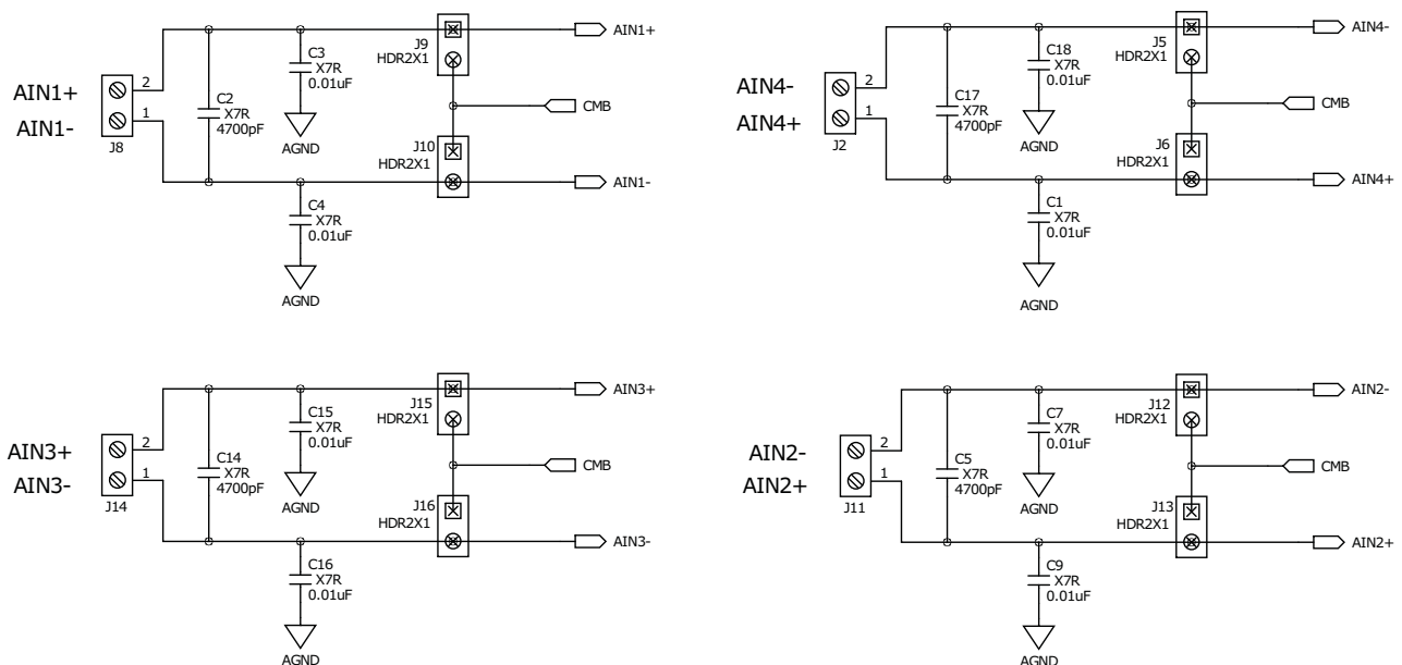
Figure 7. Analog Inputs
