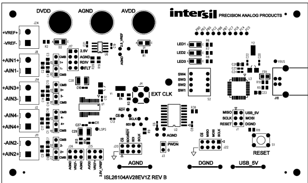
Figure 35. Component Placement
