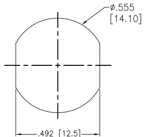
RECOMMENDED PANEL CUT-OUT (Rear Panel mounting)
