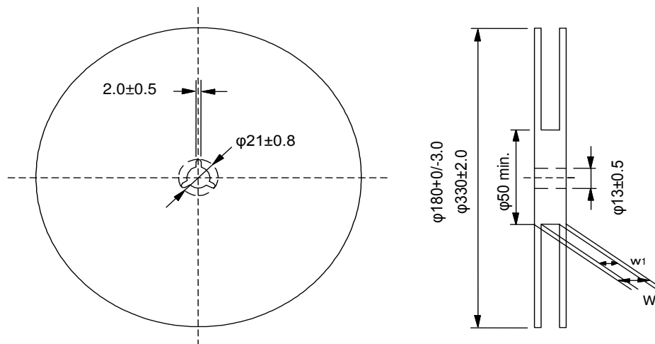
Fig.3 Taping Diagram
