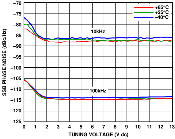
Figure 14. SSB Phase Noise vs. Tuning Voltage
