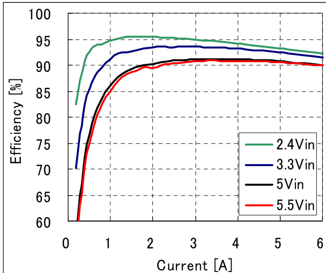
Fig-1.8V-2: Efficiency vs. load current and input voltage for Vout=1.8V. Airflow rate=200 LFM (1.0m/s) and Ta=25°C.
