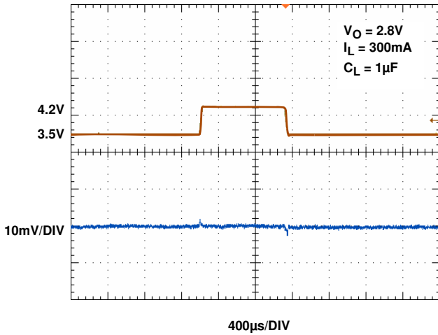
FIGURE 13. LINE TRANSIENT RESPONSE, 2.8V OUTPUT
