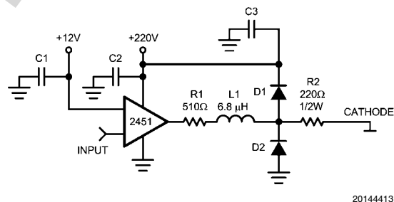
FIGURE 13. One Channel of the LM2451 with the Recommended Application Circuit
