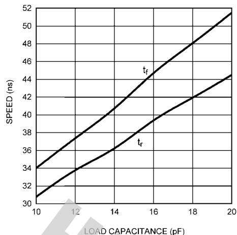
FIGURE 7. Speed vs Load Capacitance
