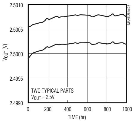
MAX6126B_25 LONG-TERM STABILITY vs. TIME (MAX)
