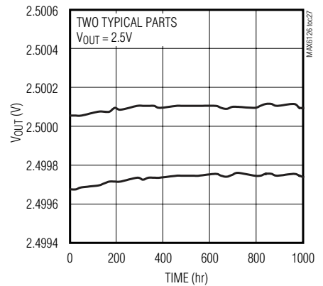
MAX6126B_25 LONG-TERM STABILITY vs. TIME (SO)
