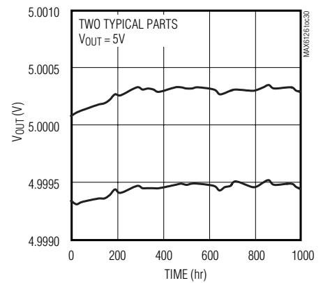
MAX6126B_50 LONG-TERM STABILITY vs. TIME (MAX)
