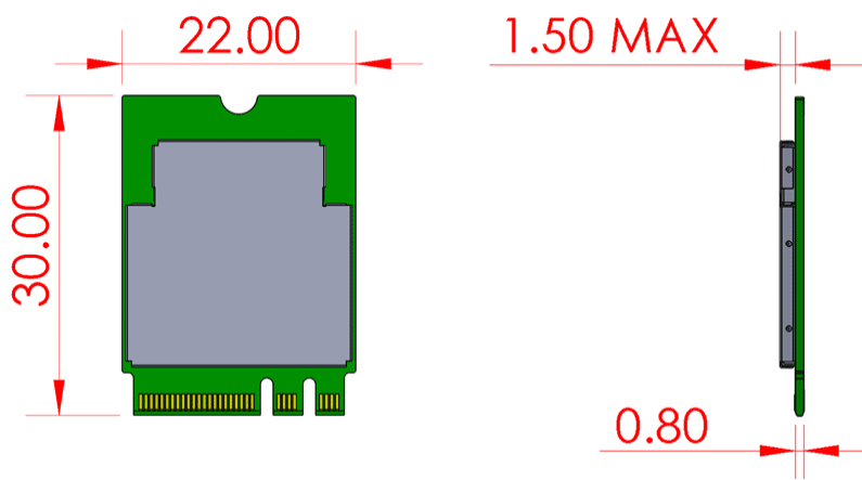
Figure 1. M.2 A+E key dimensions (in millimeters)
