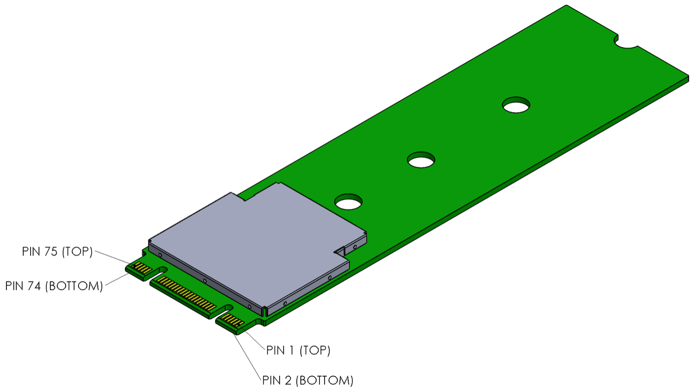
Figure 4. M.2 B+M key pin positions
