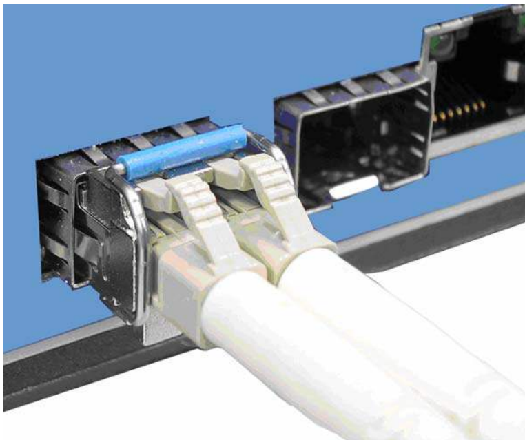
Figure 2.5-3 LC connector to the transceiver
