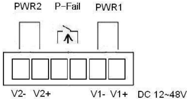
Figure 2.6-1 Pinouts of the Power Connector
