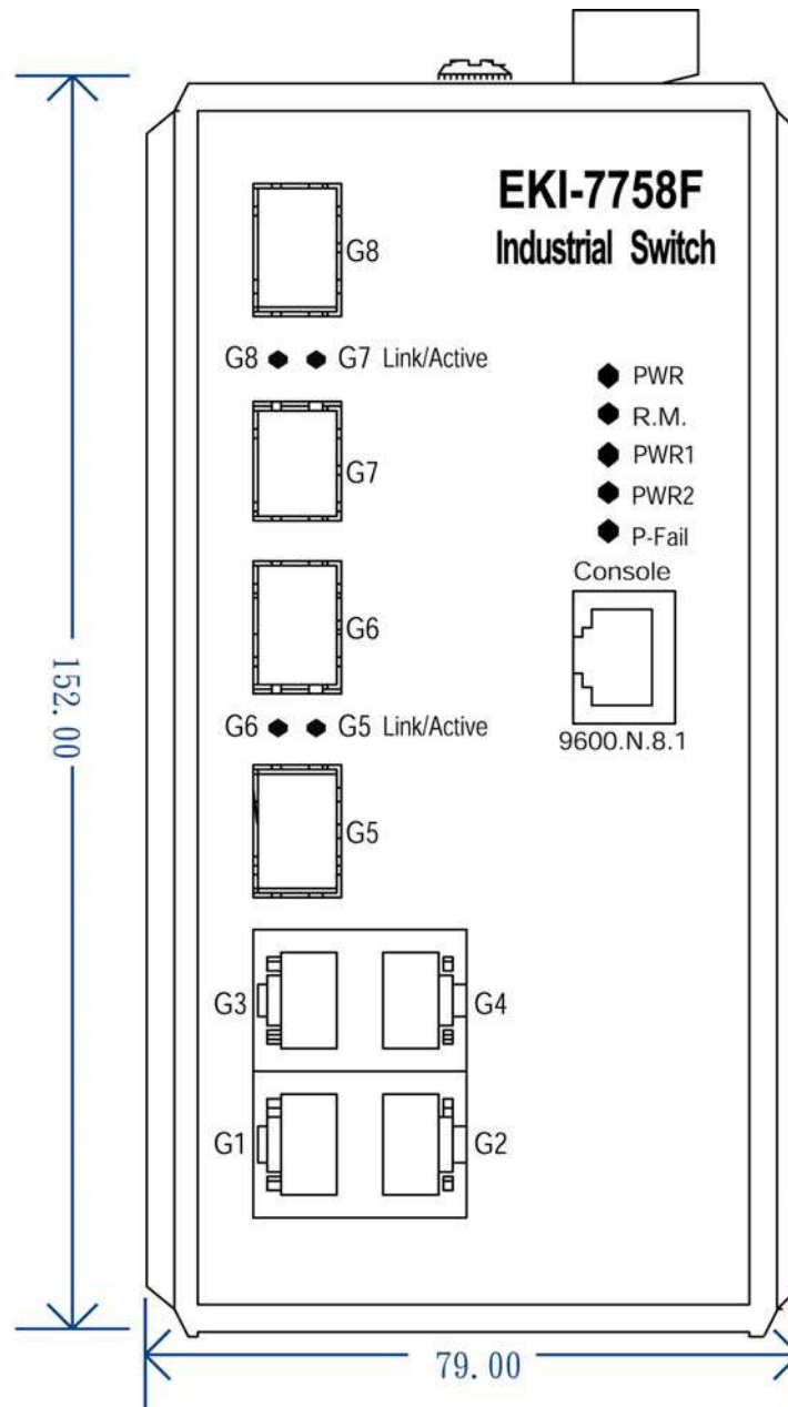
Figure 2.2-1 Front View of EKI-7758F
