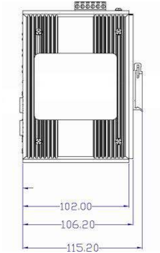
Figure 2.2-2 Side View of EKI-7758F
