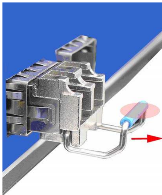
Figure 2.5-5 Pull out from the transceiver
