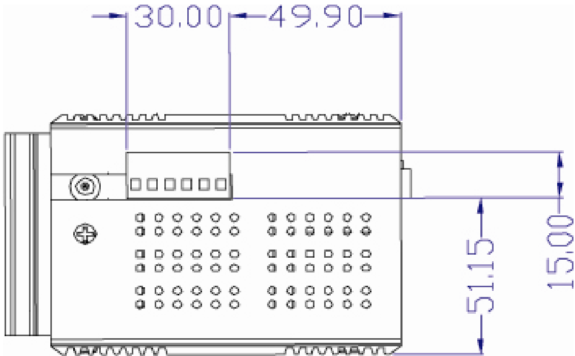
Figure 2.2-4 Top View of EKI-7758F
