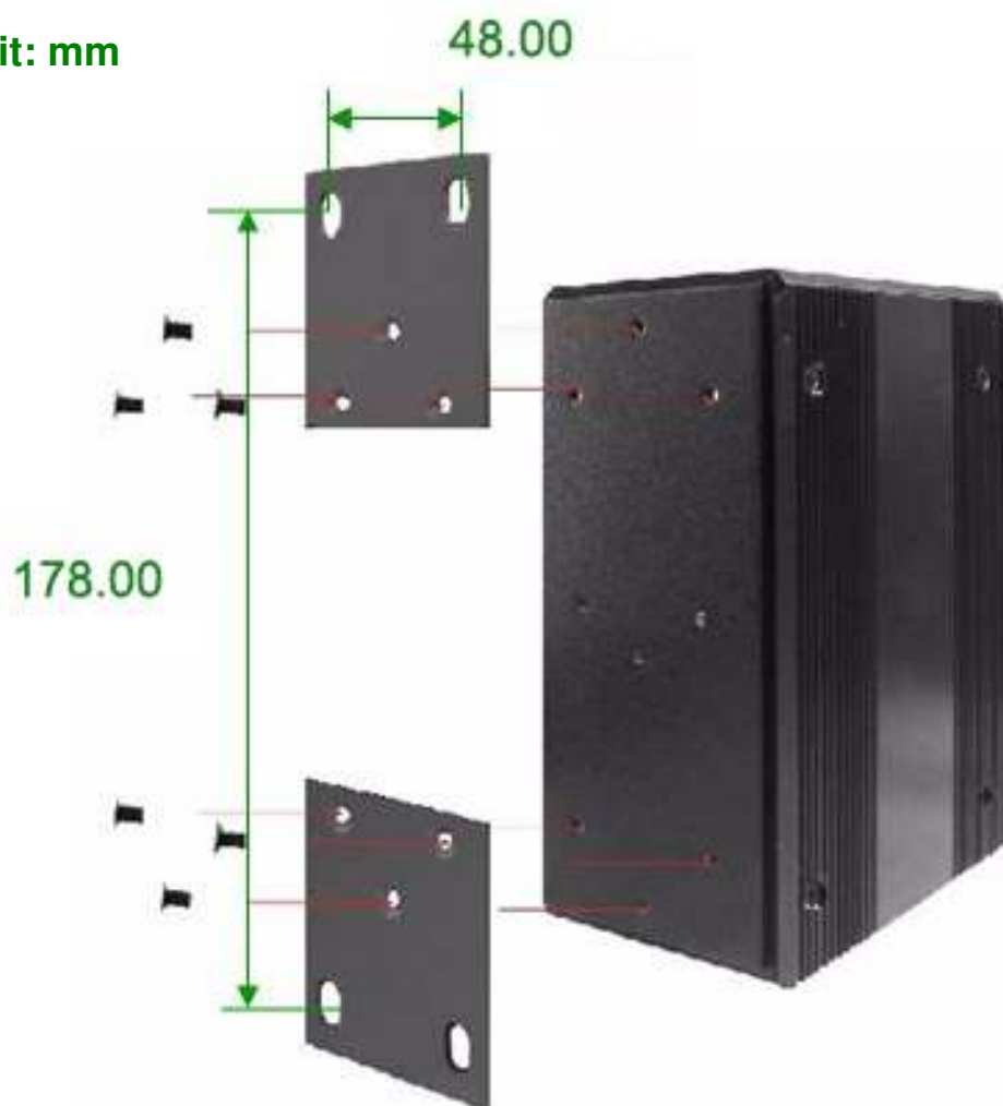
Figure 2.3-1 Combine the Metal Mounting Kit
