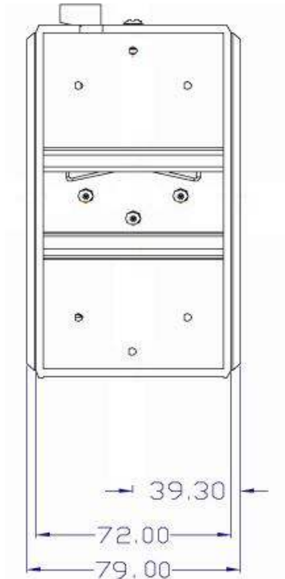
Figure 2.2-3 Rear View of EKI-7758F
