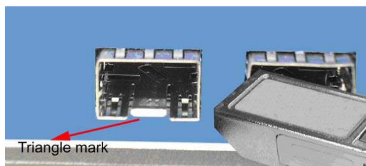
Figure 2.5-1 Transceiver to the SFP slot
