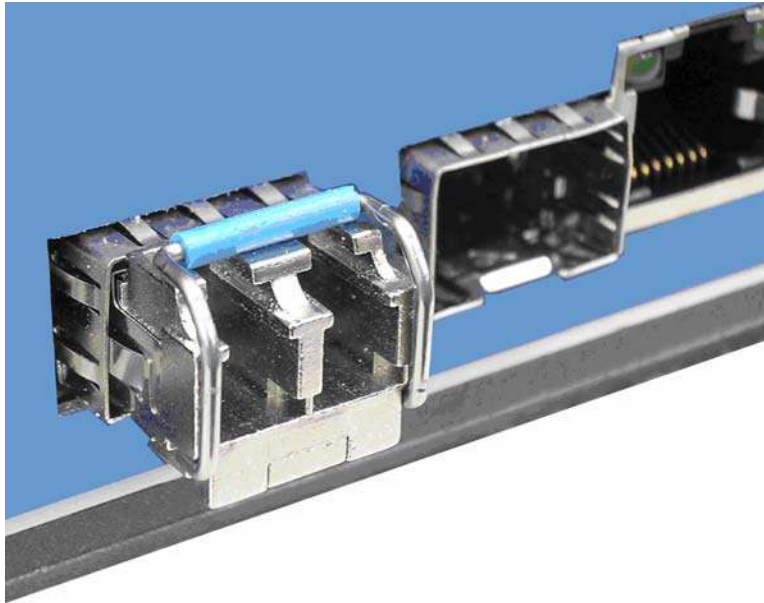
Figure 2.5-2 Transceiver Inserted
