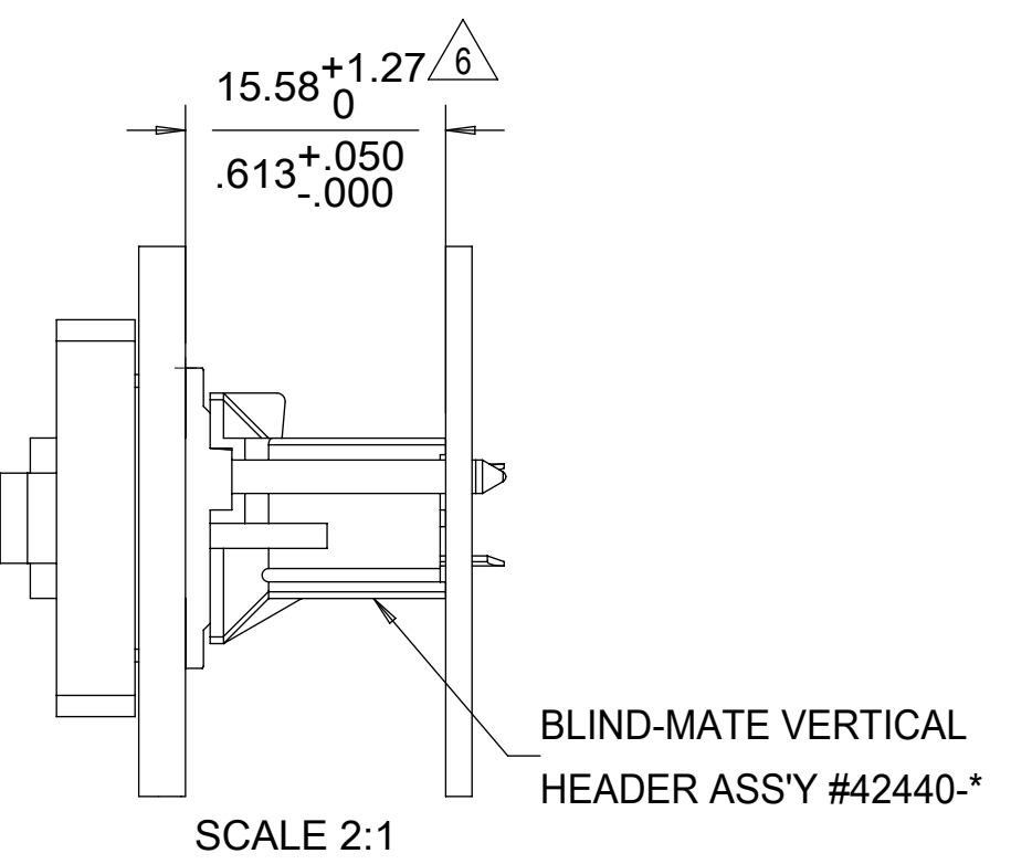
SCALE 2:1 PANEL-TO-P.C. BOARD APPLICATION #2
