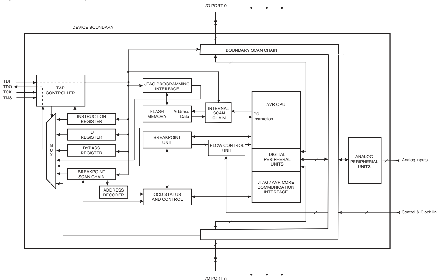
Figure 21-1. Block Diagram
