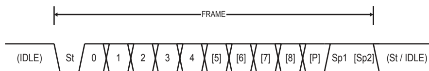
Figure 16-4. Frame Formats
