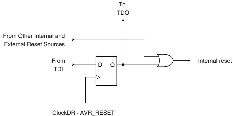
Figure 22-2. Reset Register
