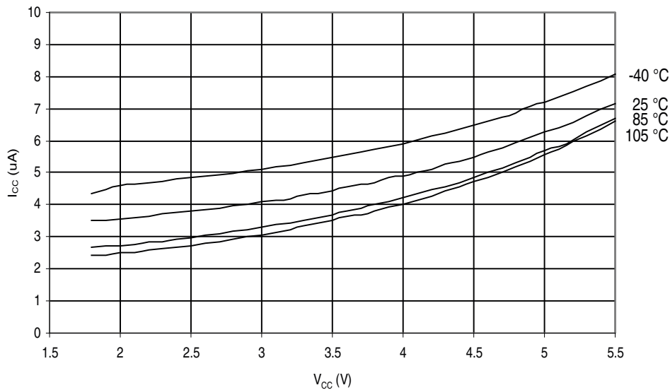
Figure 28-38. ATmega164P: Watchdog Timer Current vs. V_{CC}
