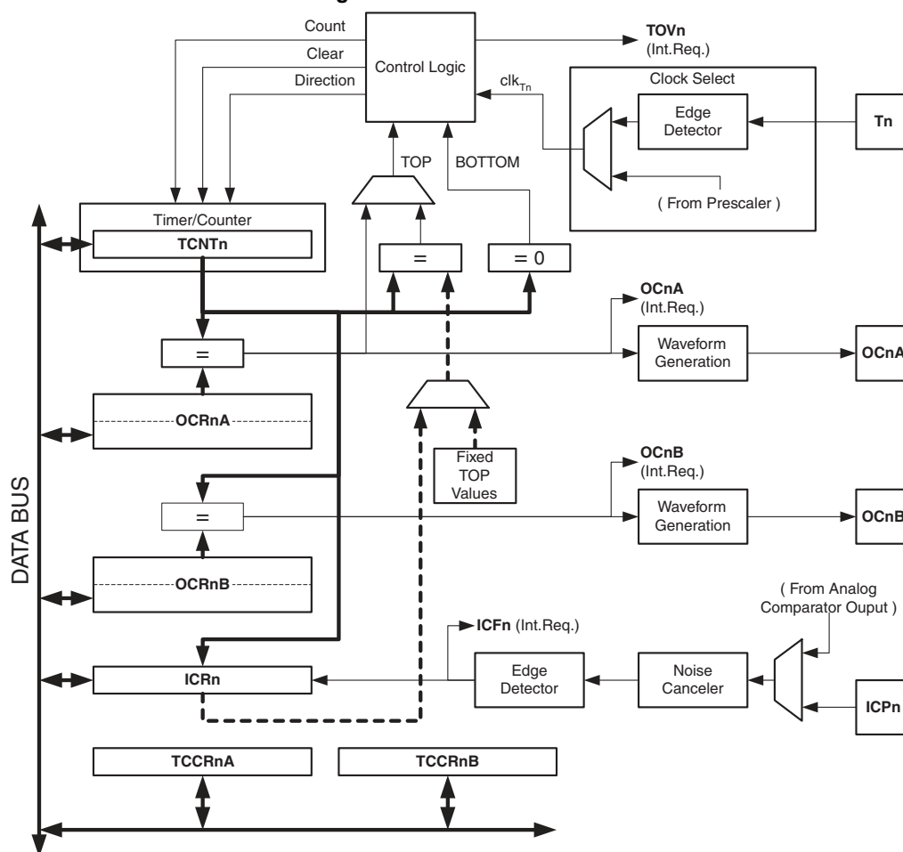
Figure 13-1. 16-bit Timer/Counter Block Diagram (1)
