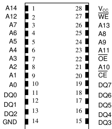
28-Pin ENCAPSULATED PACKAGE 740-mil EXTENDED
