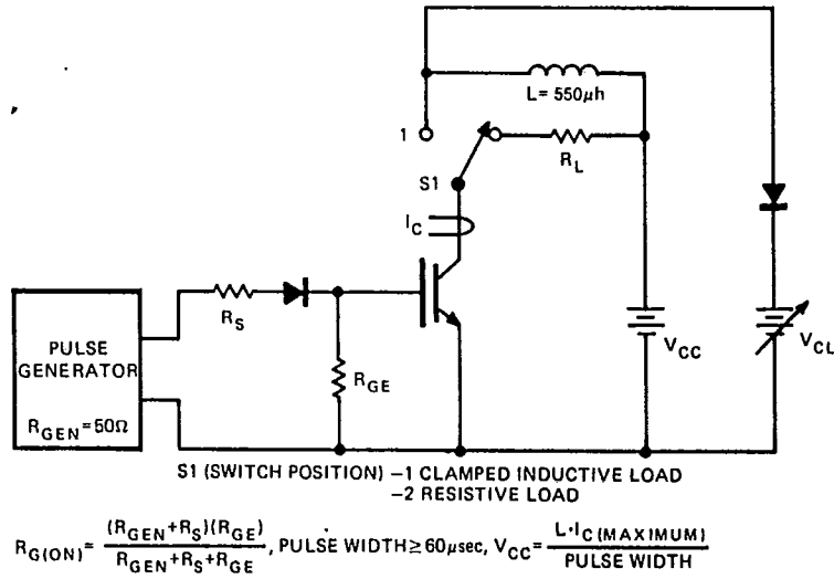
FIGURE 8. BASIC SWITCHING TEST CIRCUIT
