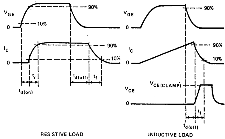
FIGURE 9. SWITCHING WAVEFORMS
