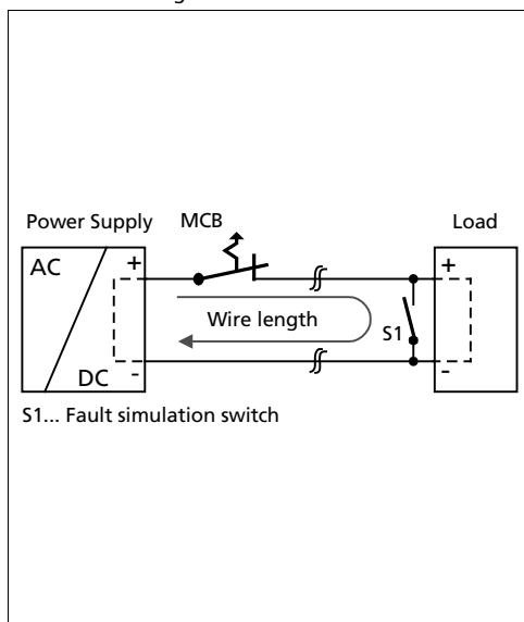
Fig. 26-9 Test circuit
