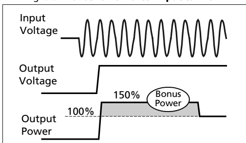
Fig. 6-6 BonusPower® after input turn-on
