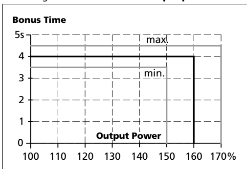
Fig. 6-3 Bonus time vs. output power
