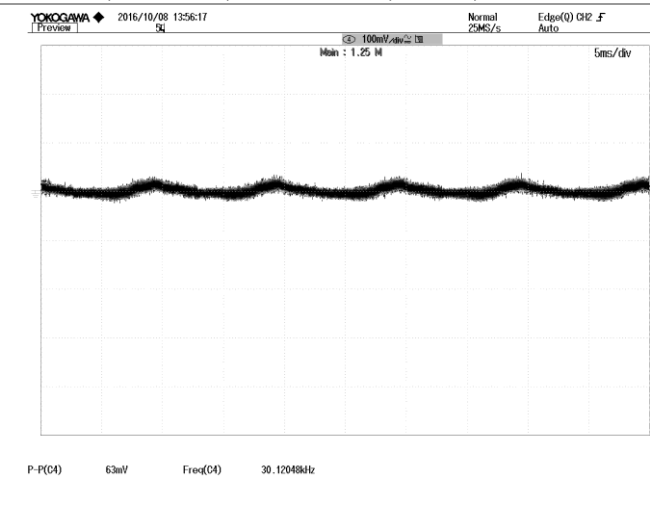
Figure 6: Output ripple & noise at 110/220Vac, 42A Iout CH3: Vout, 100mV/div, 5mS/div
