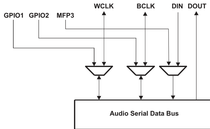
Figure 31. Alternate Audio Bus Multiplexing Function
