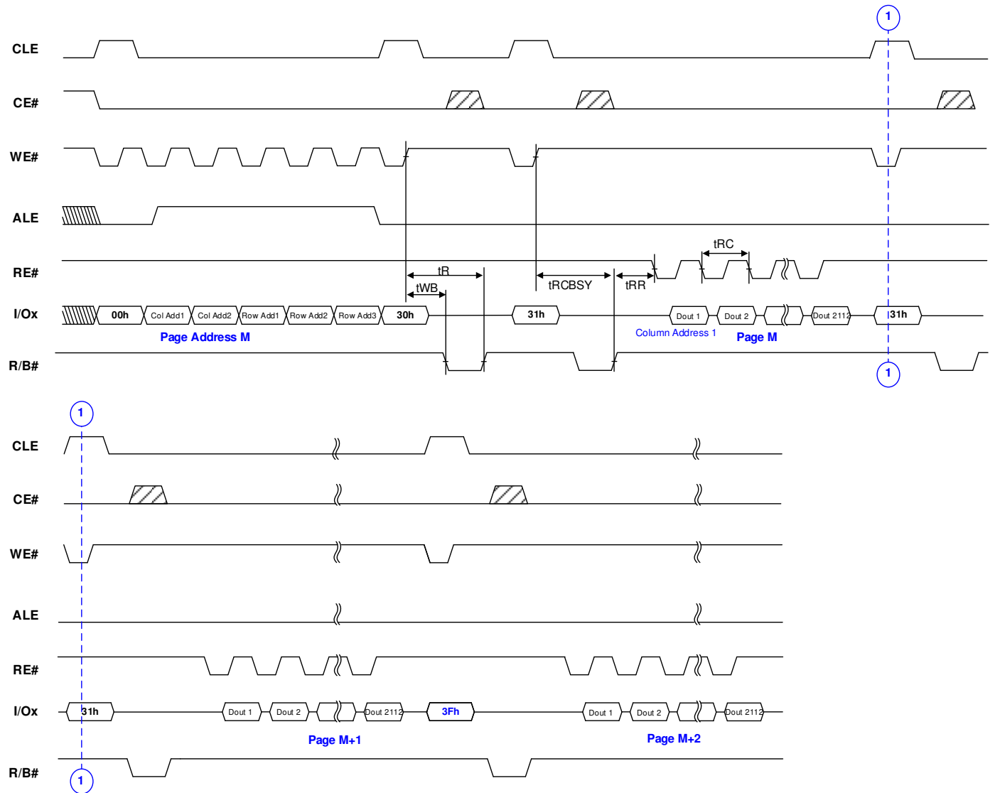
Figure 6.15.Cache Read Operation
