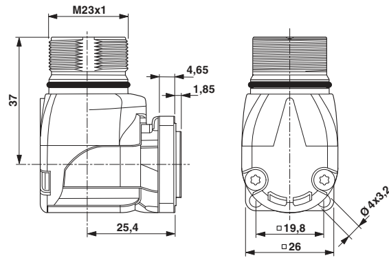
Dimensioned drawing
