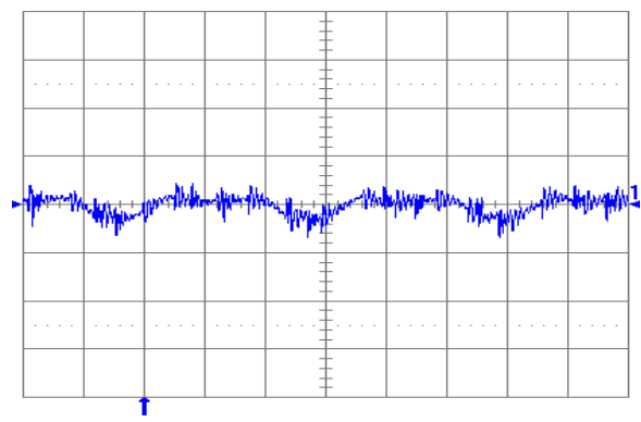
Fig. 1.2V.6: Output voltage ripple (20 mV/div.) at full rated load current into a resistive load with external capacitance 47 \mu\text{F} ceramic + 1 \mu\text{F} ceramic, and V_{in} = 5 V for V_{out} = 1.2 V. Time scale: 2 \mu\text{s} /div.
