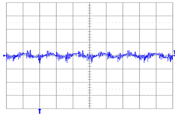
Fig. 1.5V.6: Output voltage ripple (20 mV/div.) at full rated load current into a resistive load with external capacitance 47\text{ }\mu\text{F} ceramic + 1\text{ }\mu\text{F} ceramic, and V_{in} = 5\text{ V} for V_{out} = 1.5\text{ V} . Time scale: 2 \mu\text{s} /div.
