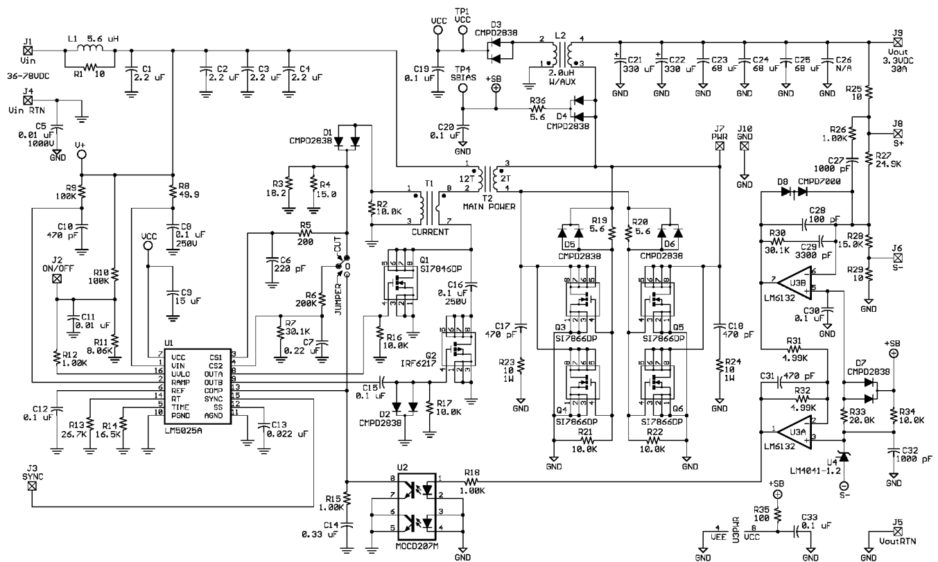
Figure 22. Application Circuit
