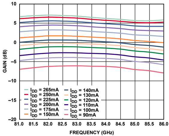
Figure 29. Gain vs. Frequency at Various Drain Currents, P_{IN} = -5 dBm/Tone, V_{CTL1}/V_{CTL2} = -1 V, Drain Current = ( I_{DD1}/I_{DD2} fixed at 50 mA) + ( I_{DD3} to I_{DD6} Swept)
