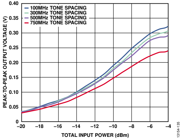
Figure 35. Envelope Detector Peak-to-Peak Output Voltage vs. Total Input Power at Various Tone Spacings, RF = 83.5 GHz, V_{CTL1}/V_{CTL2} = -5 V, V_{DET} = 4 V with 150\ \Omega Load Impedance at ENV_{DET}
