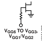
Figure 8. V_{GG6} to V_{GG3} , V_{GG1}/V_{GG2} Interface
