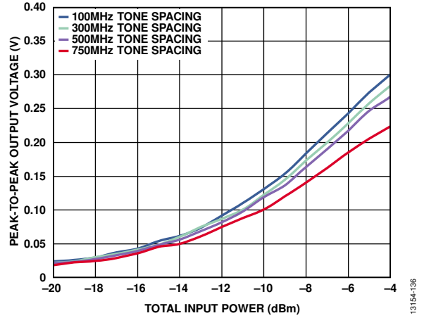
Figure 36. Envelope Detector Peak-to-Peak Output Voltage vs. Total Input Power at Various Tone Spacings, RF = 86 GHz, V_{CTL1}/V_{CTL2} = -5 V, V_{DET} = 4 V with 150\ \Omega Load Impedance at ENV_{DET}
