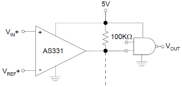
Driving CMOS
