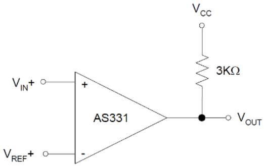
Basic Comparator
