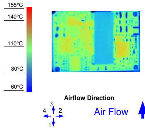
Figure 8. Thermal Image for Airflow Direction 3 (7.5A output, 55°C ambient, 200 LFM, typical Vin, open frame, unit soldered onto a fixture board)
