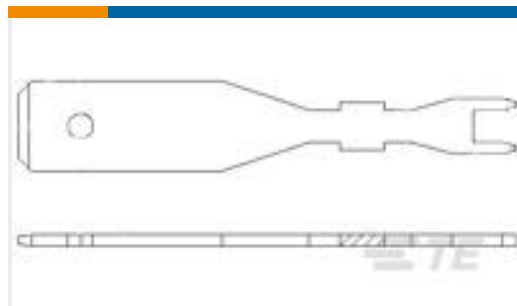
TE Part #1217742-1 250 FASTON,PCB TAB,TNBR
