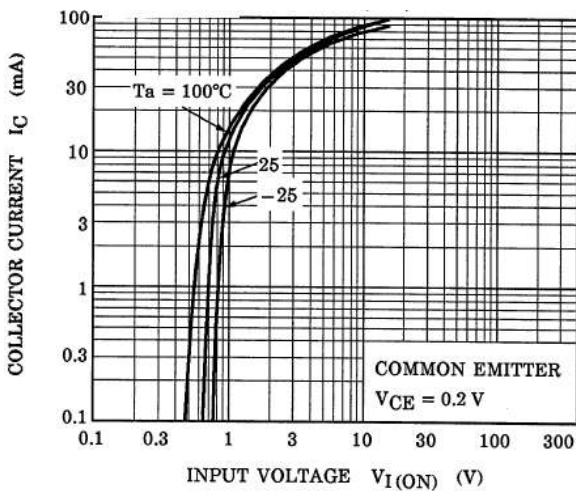
Fig. 10.5 RN1405 I_C - V_{I(ON)}
