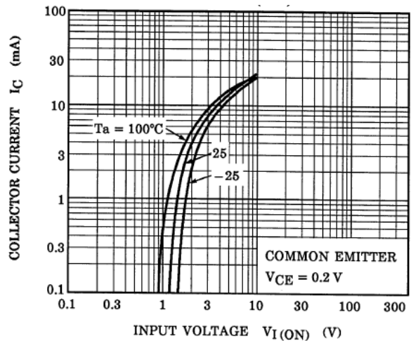
Fig. 10.4 RN1404 I_C - V_{I(ON)}
